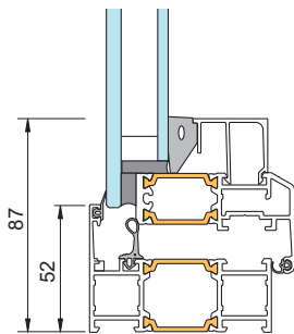
1. Liten karm/båge
